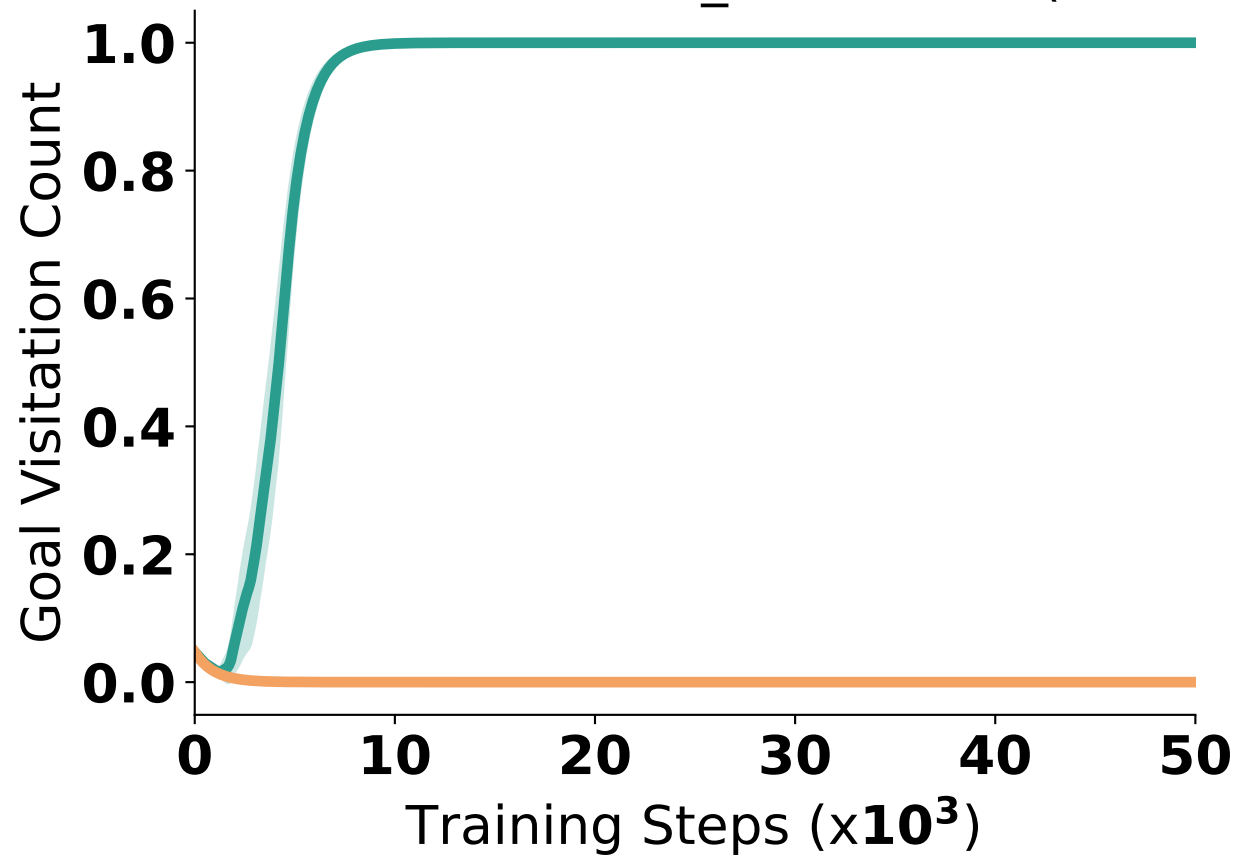
Gridworld-Bottleneck_FullRandom(20.0%)
